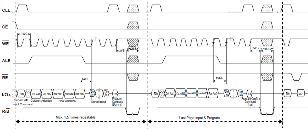
Figure 21 : cache program
